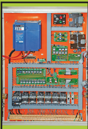
MICROPROCESSOR V3F CONTROLLER
